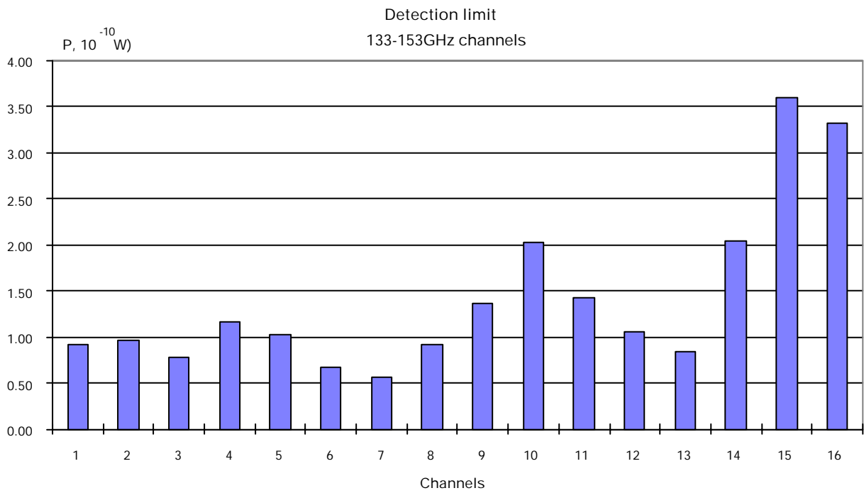
Fig. 4. Detection limit for 16 channels covering 133-153 GHz band.
