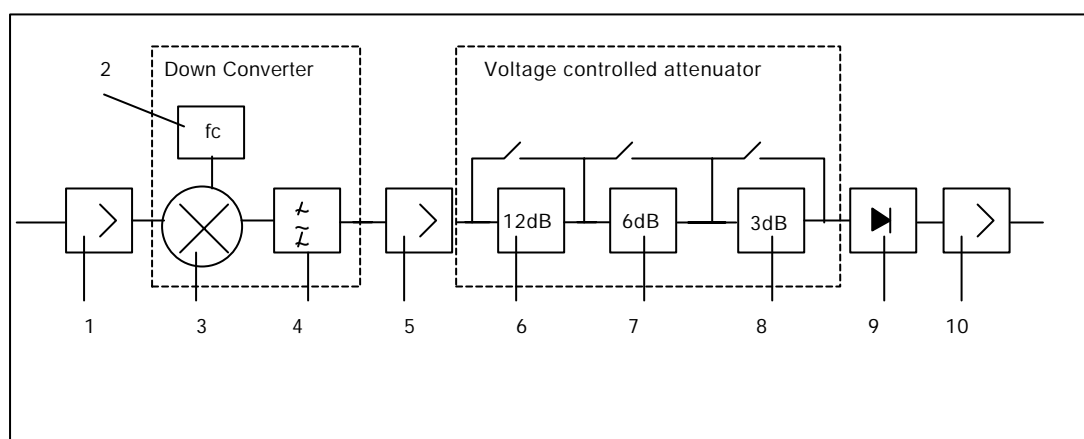
Fig. 12. Module of the IF Block.
