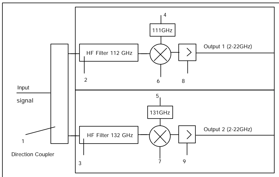
Fig. 7. Block-scheme of the RF Block.
