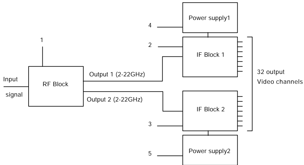
Fig. 5. Block-scheme of the Radiometer.
