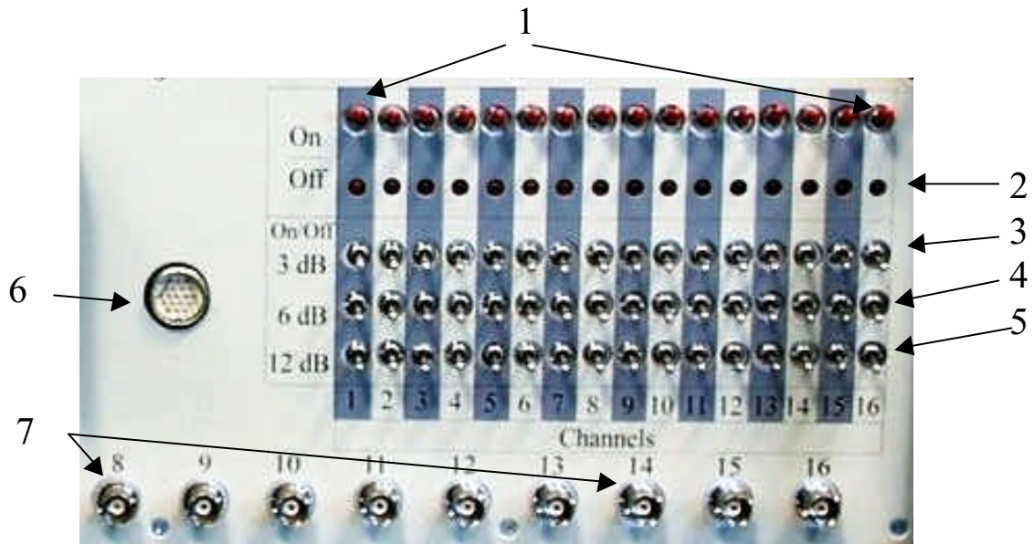
Fig. 13. Front panel of the IF Block.
